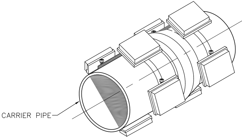
PIPE CASING DETAIL
